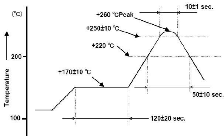
Figure 1) Suggested Reflow Profile
