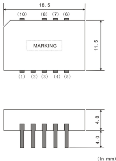
DIP10K
