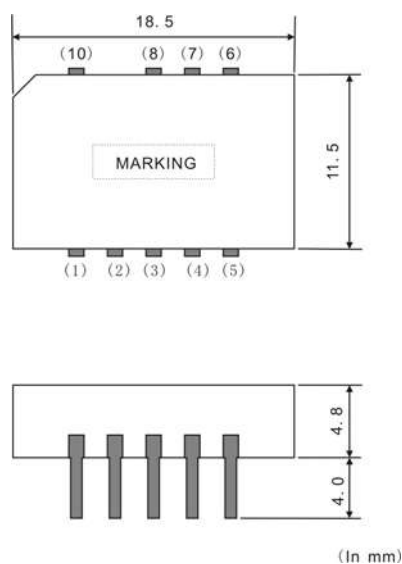
DIP10K
