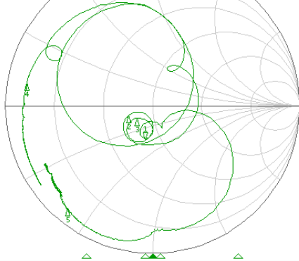
▶[F8] S11 Smith (R+jX) Scale 1.000U [F2]
