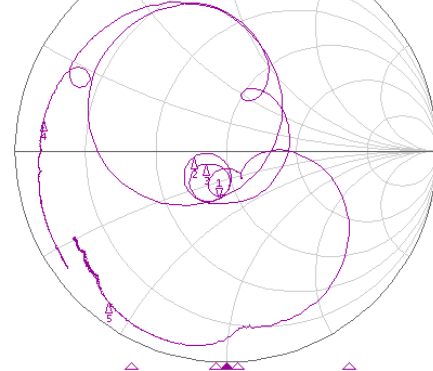
▶[F9] S22 Smith (R+jX) Scale 1.000U [F2]
