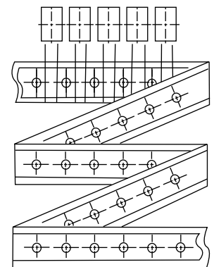
● Tape Arrange
