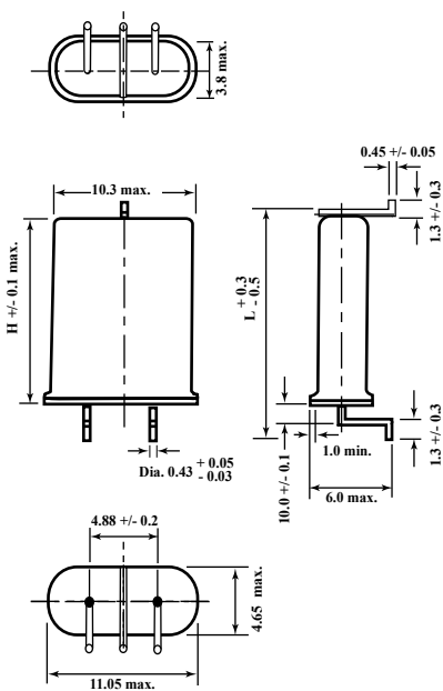
HC49U (SMD )
