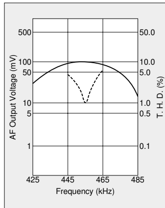
CDBC455CLX36/NE (SA) 606/616
