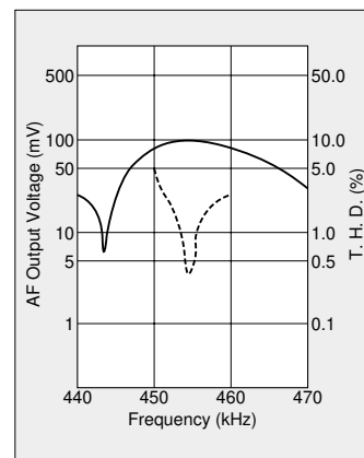
CDBC455CX29/NE605
