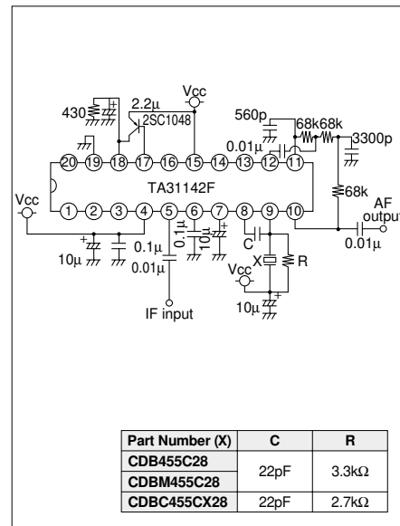
TA31142
