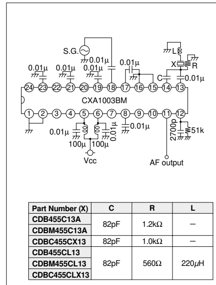
CXA1003BM
