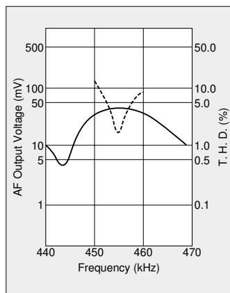
CDBC455CX40/TA31145
