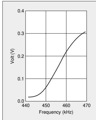
CDBM455C47/TA31147
