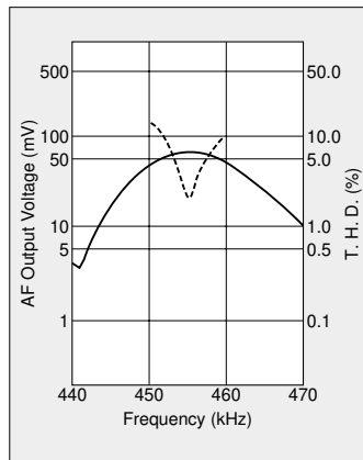
CDBM455C50/CXA3117
