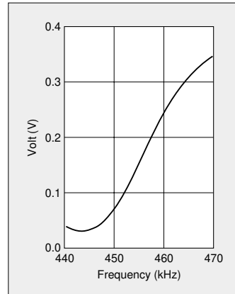
CDBC455CX54/TA31149
