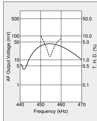
CDBM455C40/TA31145
