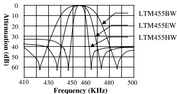
LTM455/W CHARACTERISTICS
