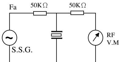
LZU TEST CIRCUIT-Fa
