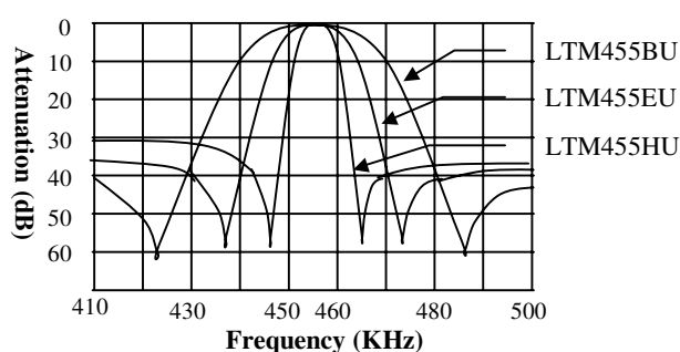
LTM455/U CHARACTERISTICS
