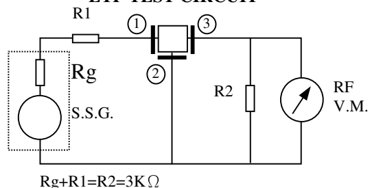
LTP TEST CIRCUIT
