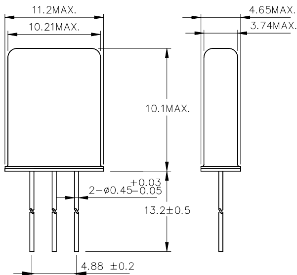
Figure 1 49/T Package
