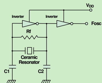
Figure 3: Oscillator Circuit
