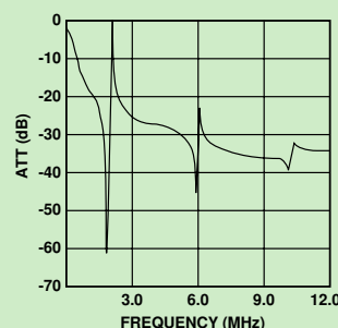
Figure 11: MHz Spurious Response
